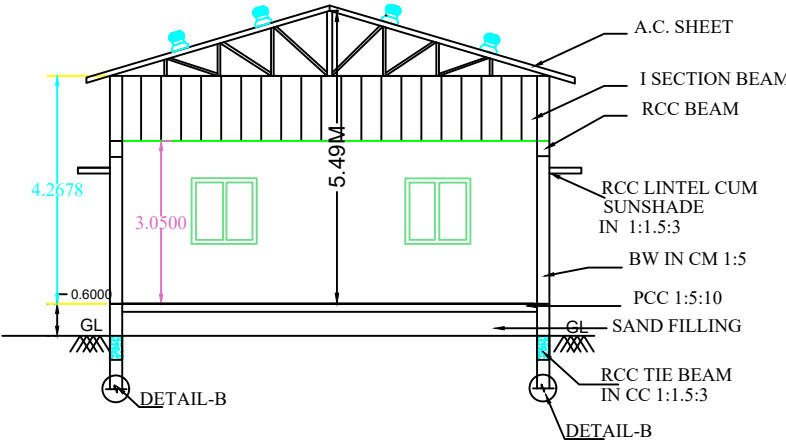
SECTION @ XY
