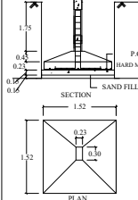
FOUNDATION DETAILS
