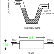
DETAILS OF "U" TRAP NOT TO SCALE
