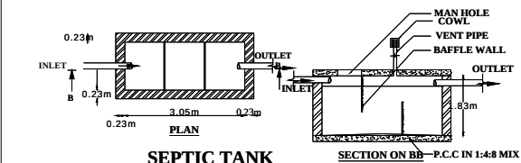
SEPTIC TANK
