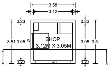
PROPOSED GROUND FLOOR PLAN
