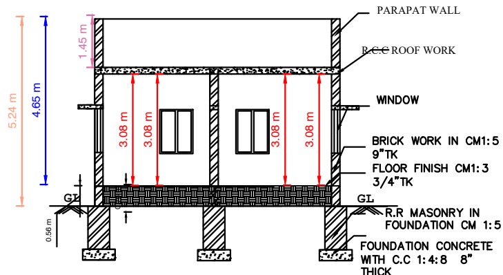
SECTION " AB "
