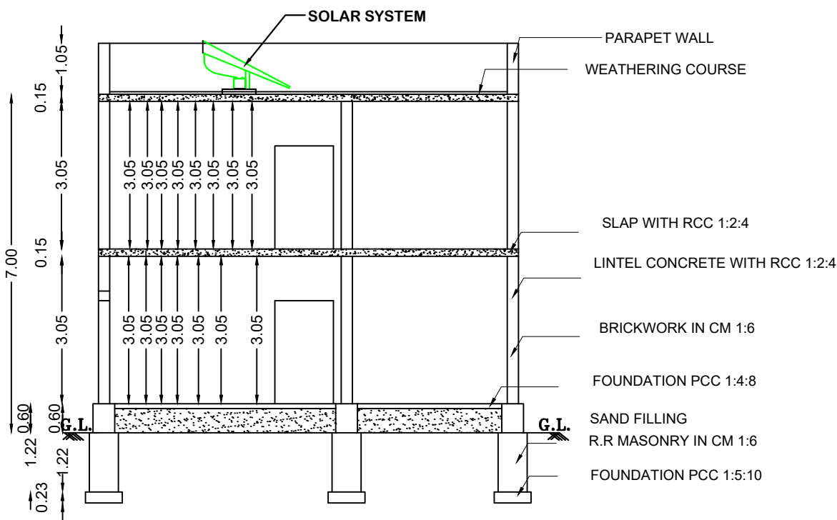
SECTION ON-'AB'
