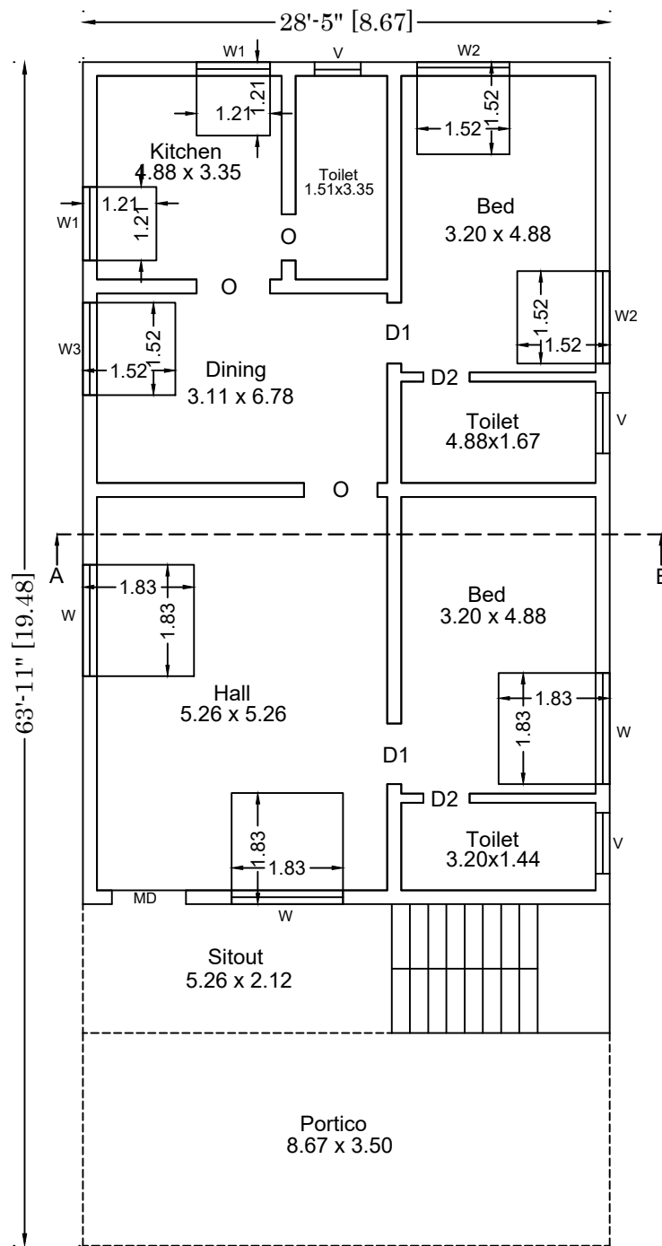
D FLOOR PLAN SCALE-1:100
