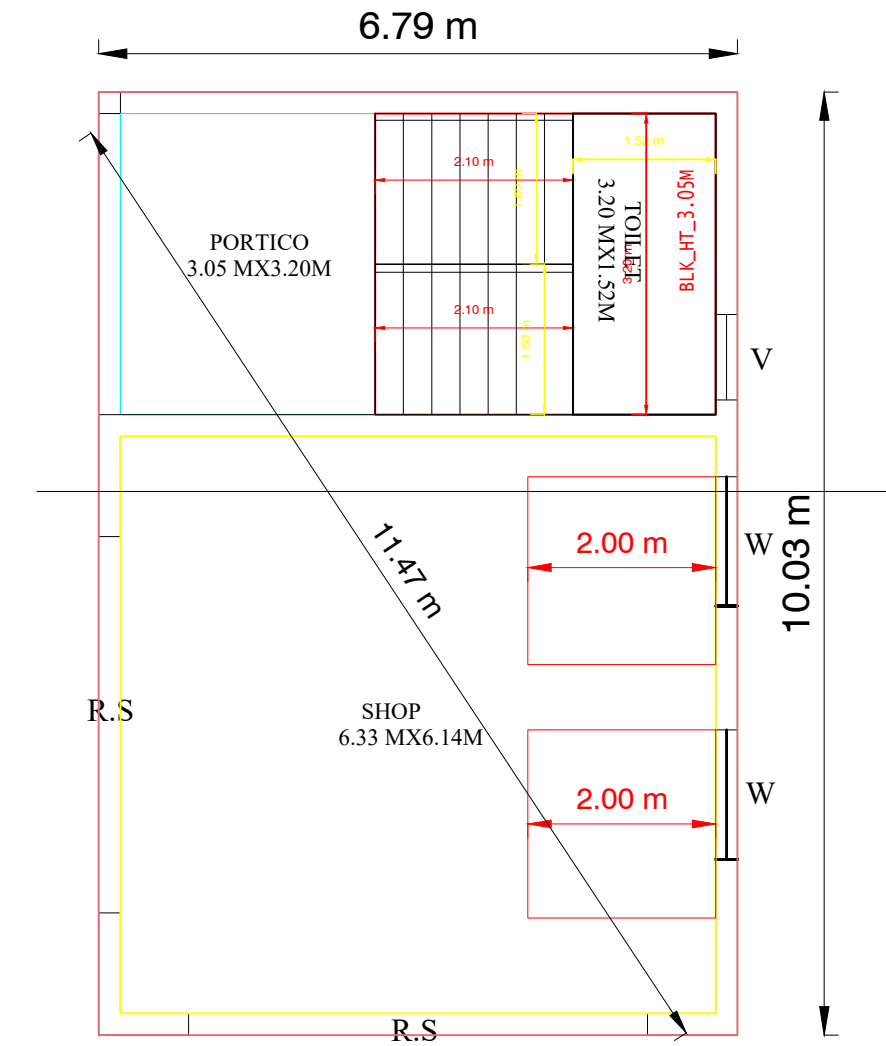
COMMERCIAL GROUND FLOOR
