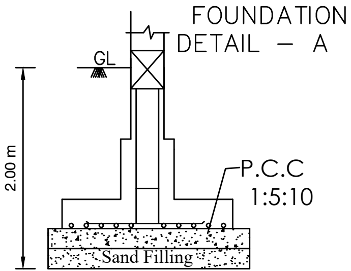
Isolated Footing -A (1.50X1.50) (Not to Scale)
