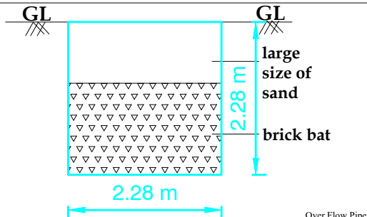
RAINWATER HARVESTING RWH TANK CAPACITY=2000LITER
