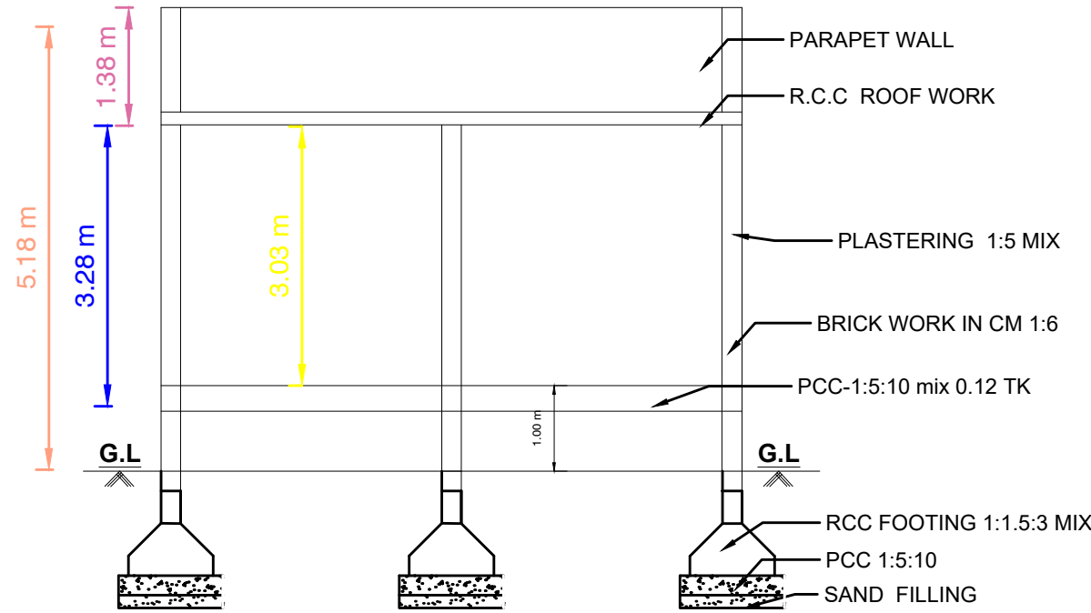
SECTION"AB"
