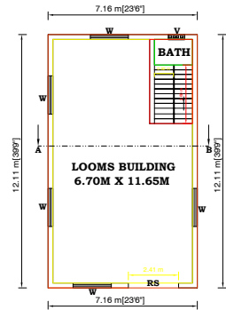
LOOMS BUILDING - PLAN
