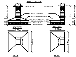
COLUMN FOOTING DETAILS
