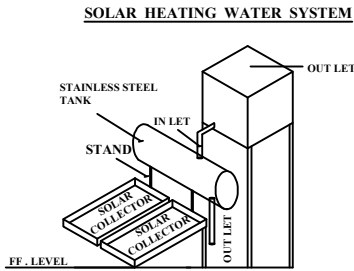
SOLAR HEATING WATER SYSTEM
