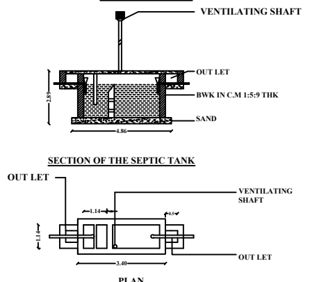
SEPTIC TANK
