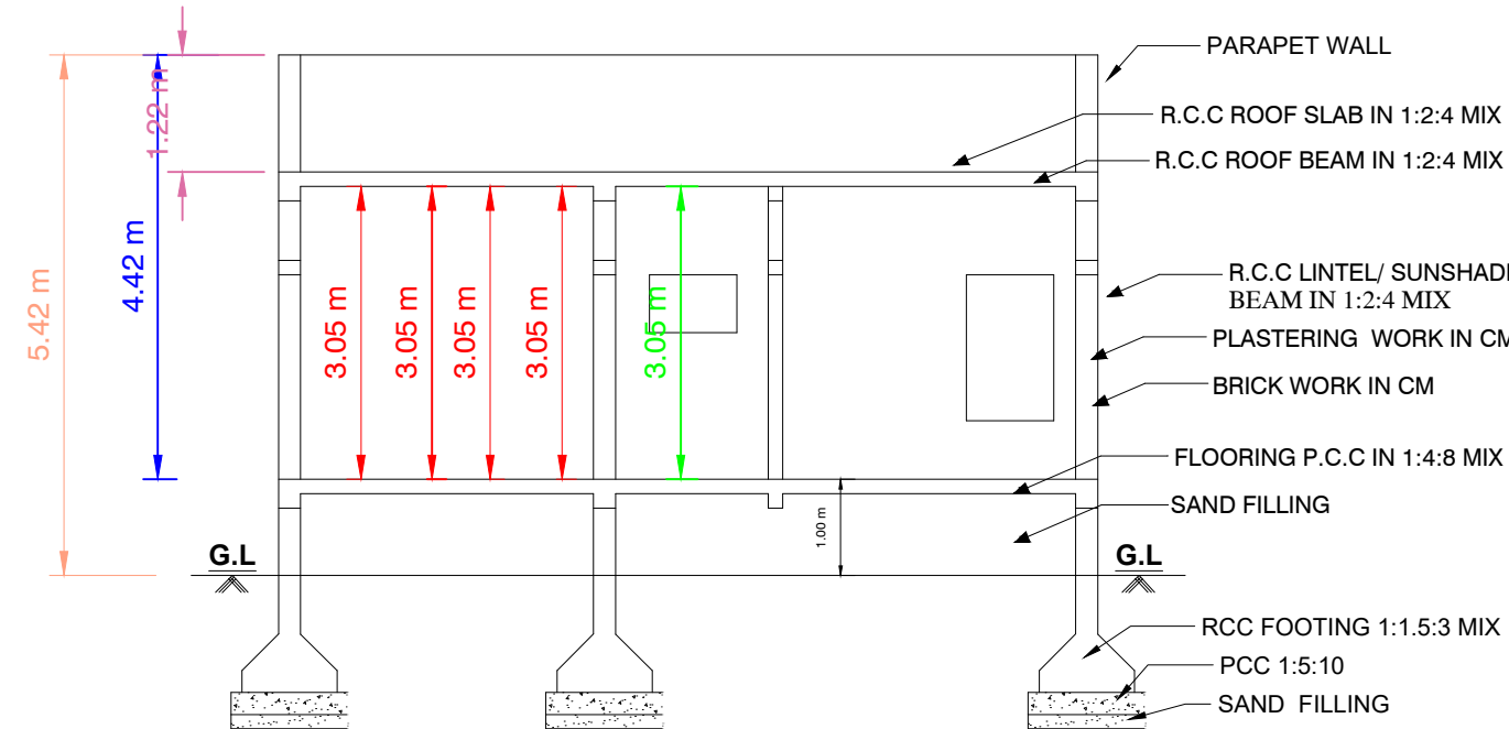
SECTION"AB"
