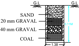
SECTION ON RAIN WATER COLL .TANK
