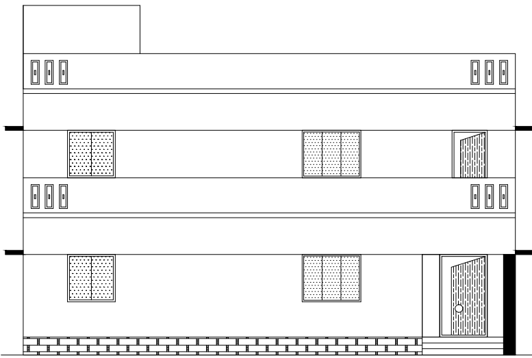
FRONT ELEVATION
