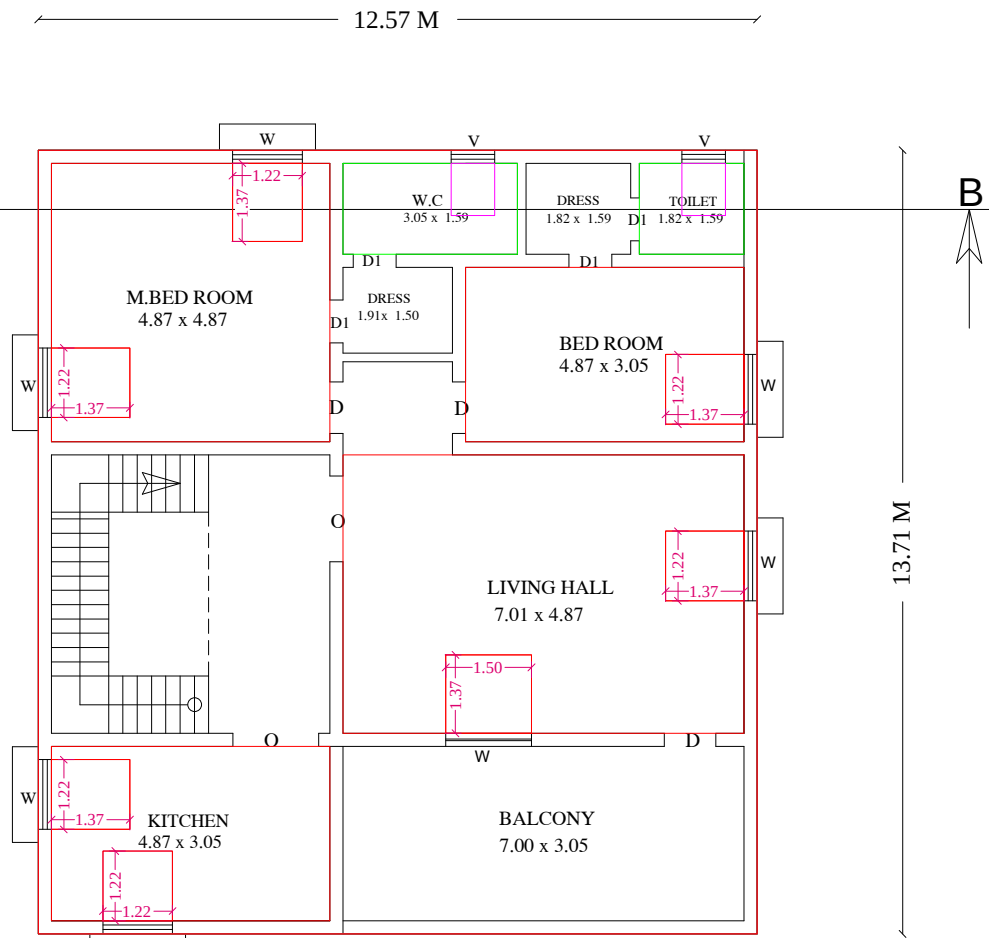
PLAN- FIRST FLOOR
