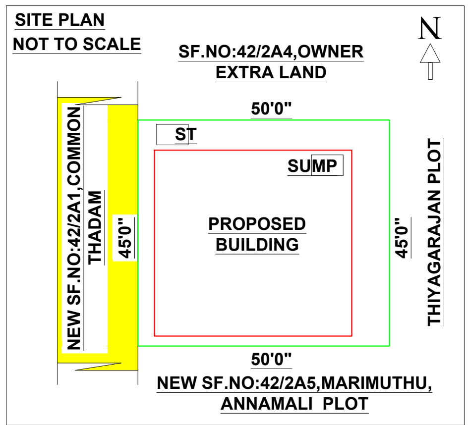
RAINWATER HARVESTING RWH TANK CAPACITY=2000LITER
