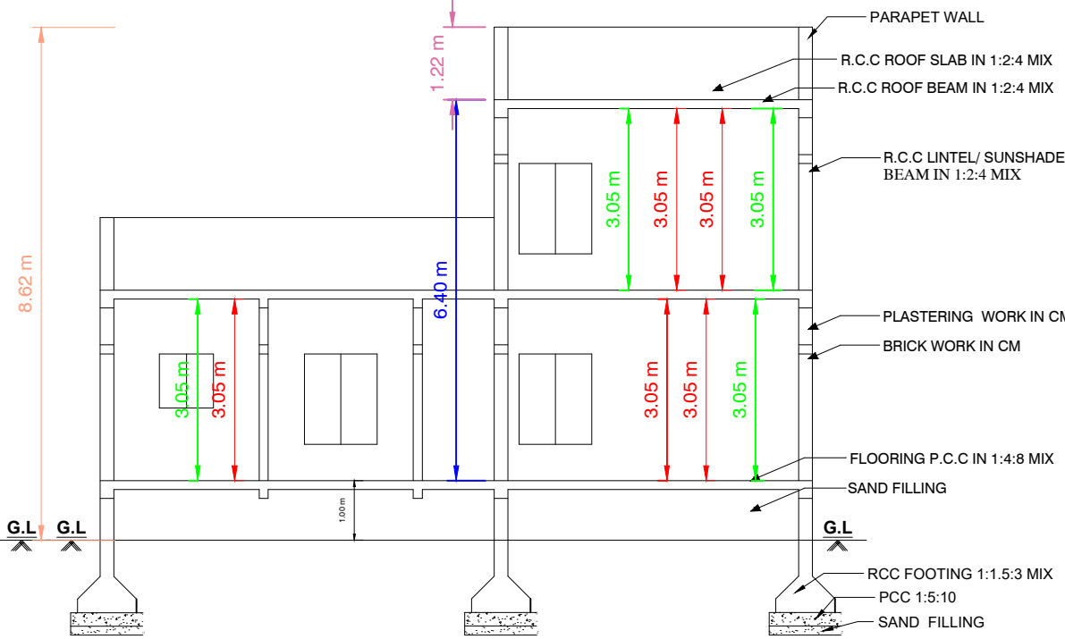
SECTION"AB"
