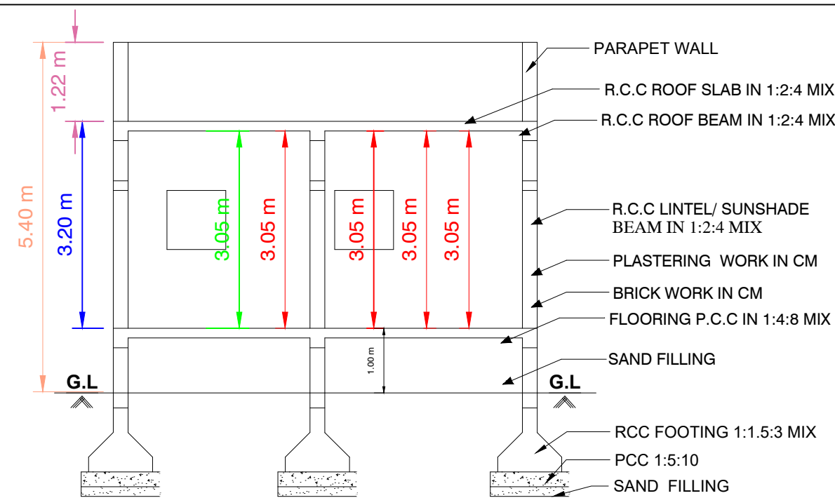
SECTION"AB"
