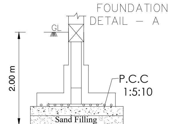
Isolated Footing -A (1.50X1.50) (Not to Scale)
