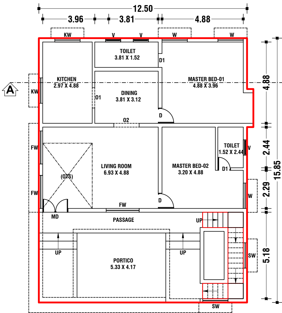
NORTH FACING GROUND FLOOR PLAN
