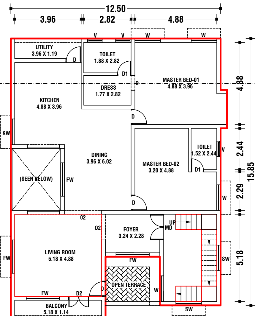
NORTH FACING FIRST FLOOR PLAN
