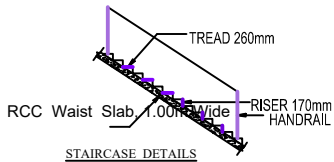
STAIRCASE DETAILS
