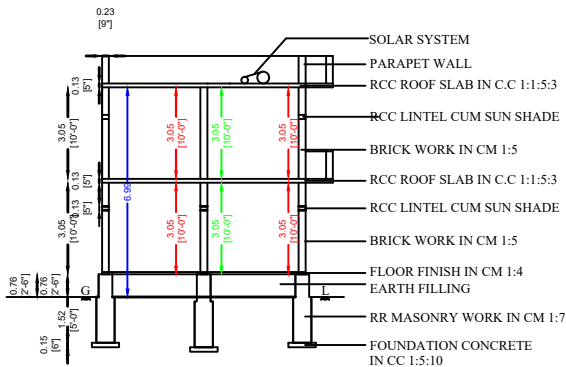
SECTION "AA","BB"
