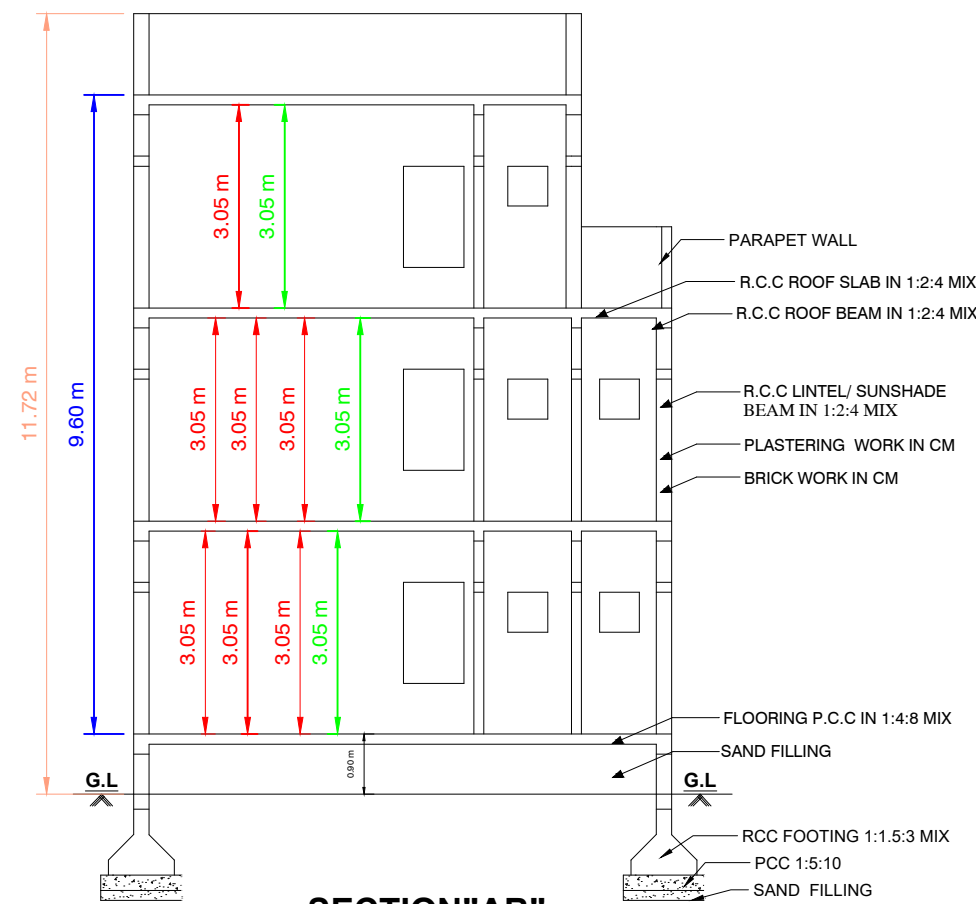
SECTION "AB"
