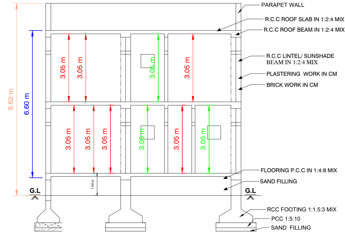
SECTION"AB"
