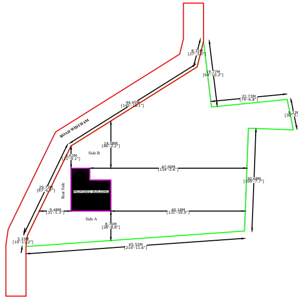
SITE PLAN
