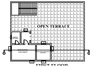
FIRST FLOOR
