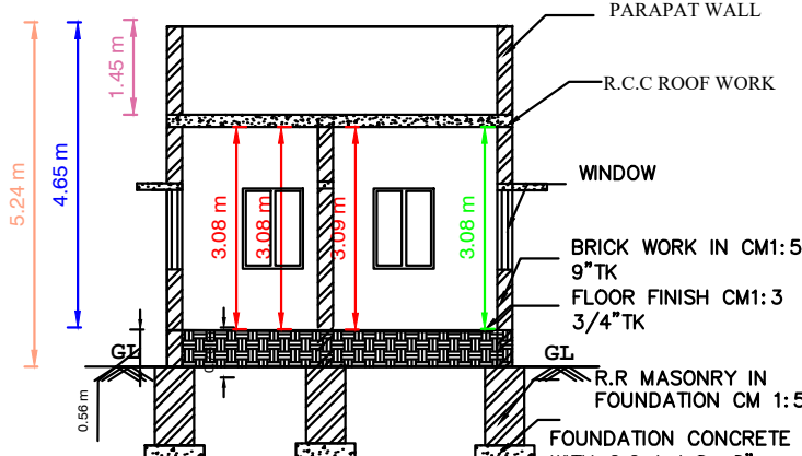
SECTION " AB "
