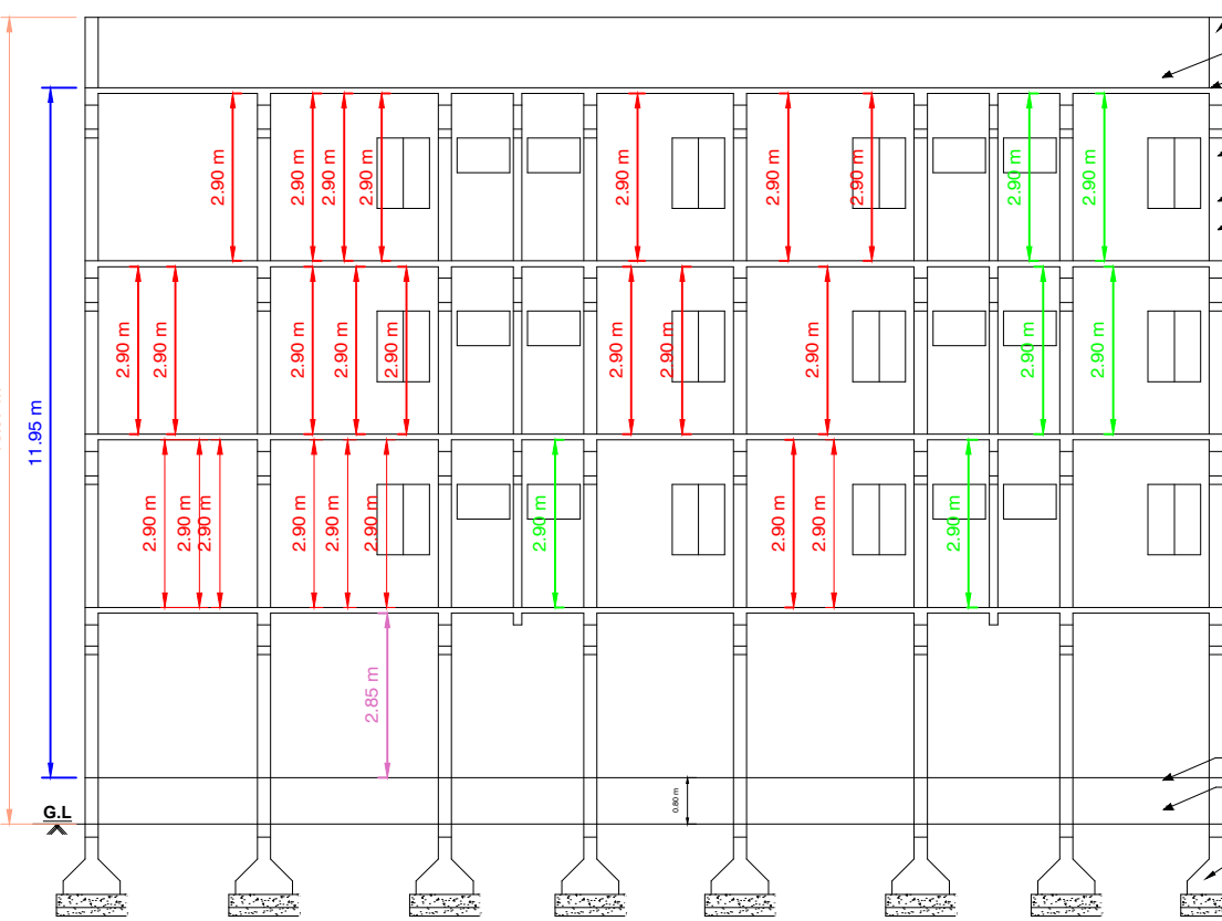
SECTION"AB"
