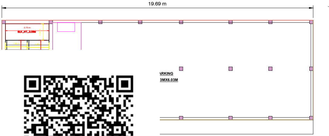
FLOOR
