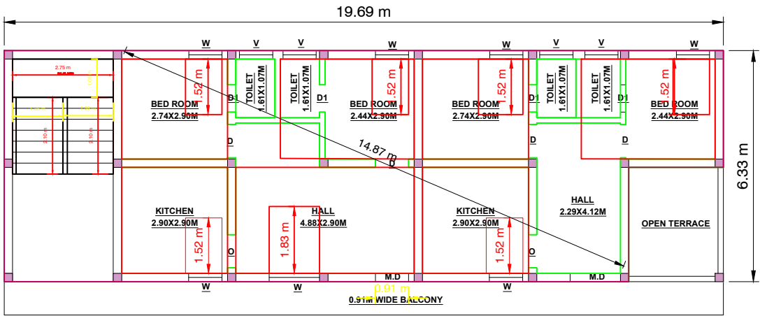
THIRD FLOOR
