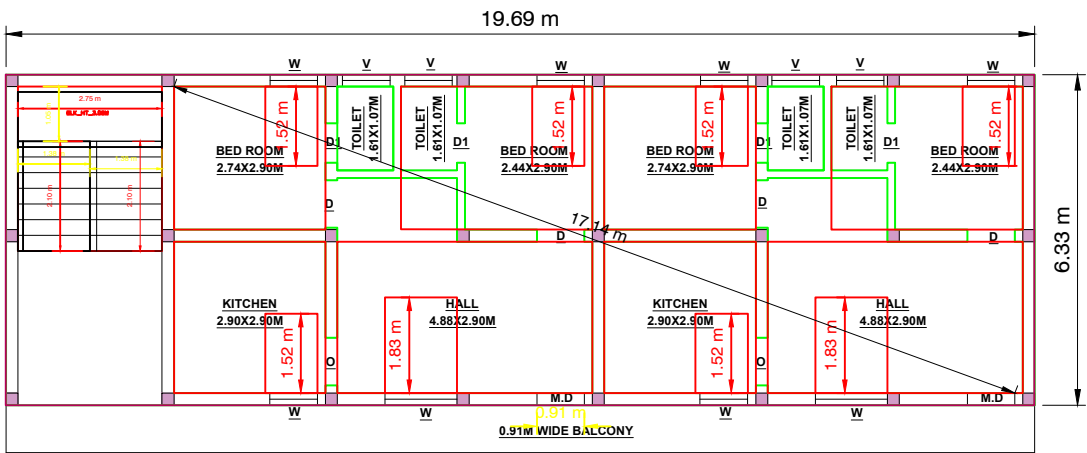
SECOND FLOOR
