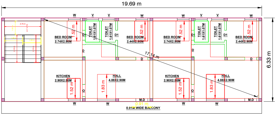
FIRST FLOOR
