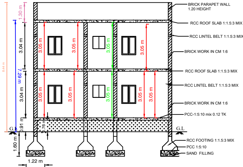
SECTION "AB"
