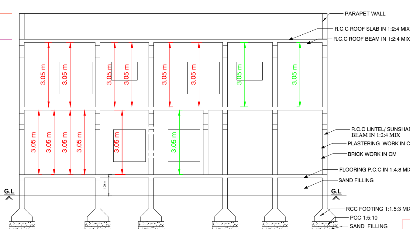
SECTION"AB"
