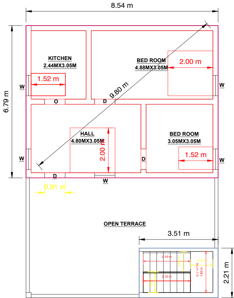
FIRST FLOOR
