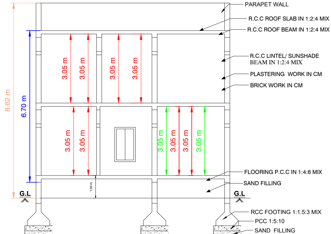
SECTION"AB"
