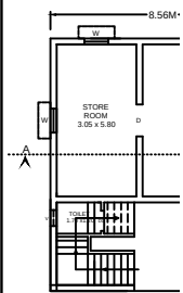
GROUND FLOOR
