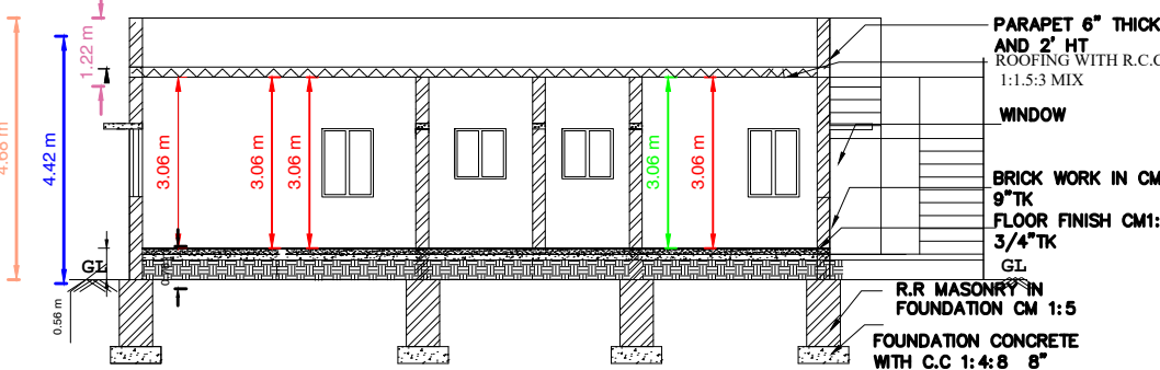
SECTION " AB "
