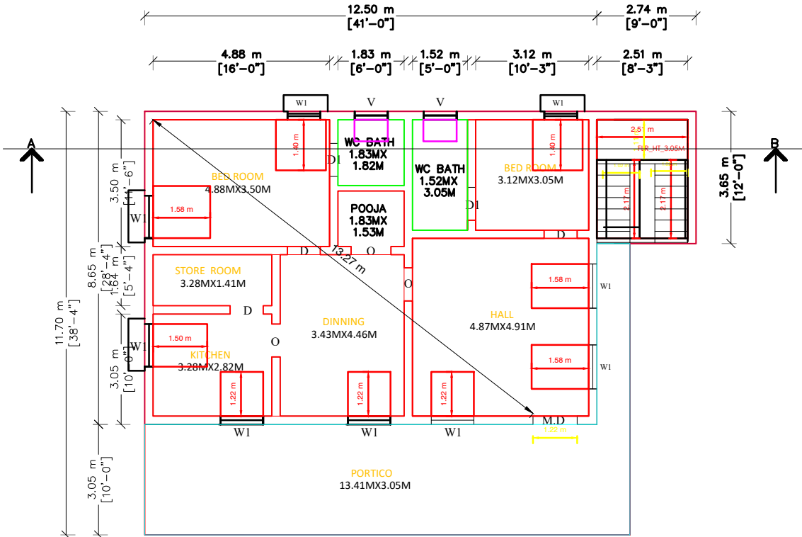
GROUND FLOOR PLAN ENTRANCE FACING TO EAST
