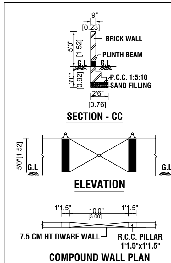
COMPOUND WALL PLAN
