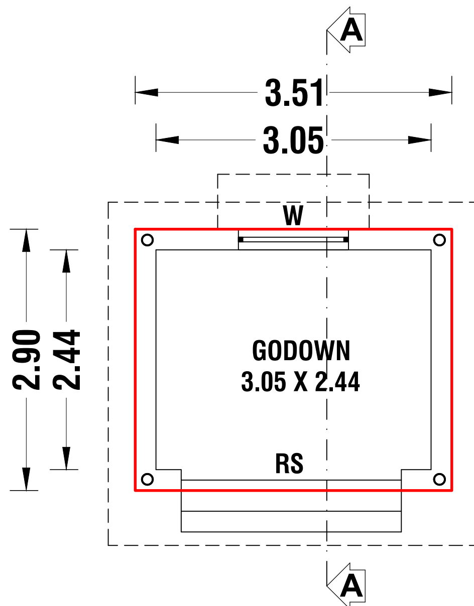
EAST FACING GROUND FLOOR PLAN
