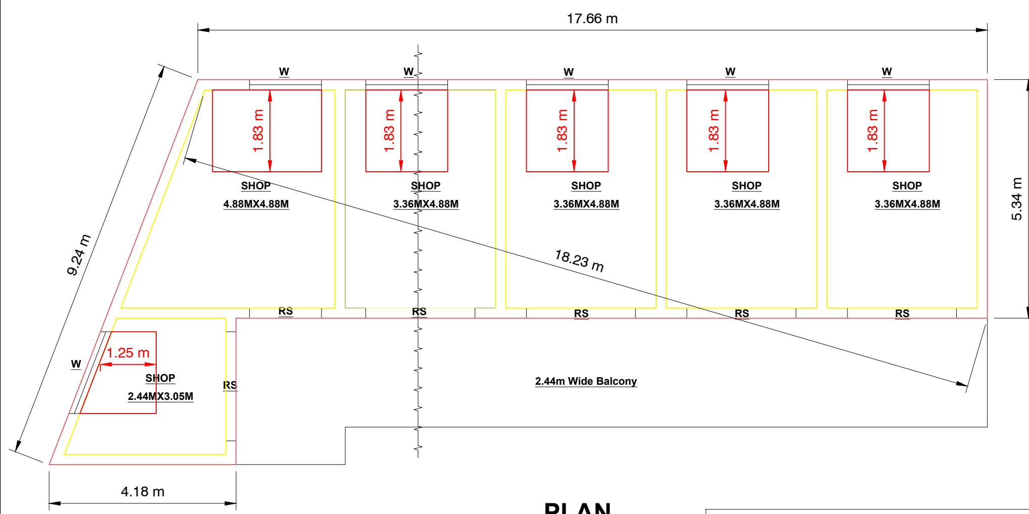
PLAN
