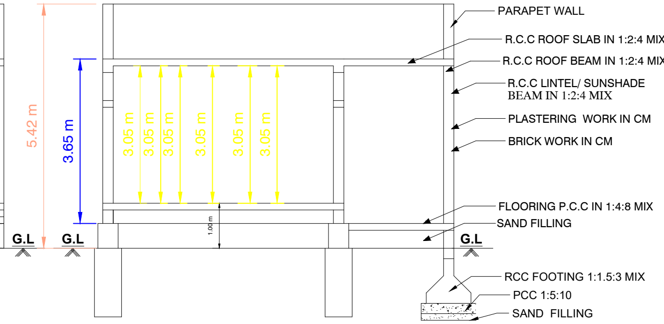
SECTION"AB"
