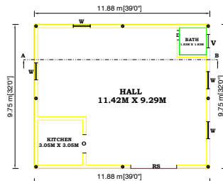
COMMERCIAL HALL - PLAN
