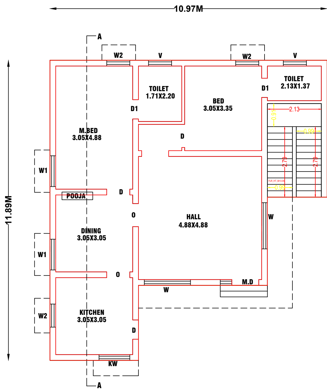
GROUND FLOOR PLAN-I (SCALE 1:100)
