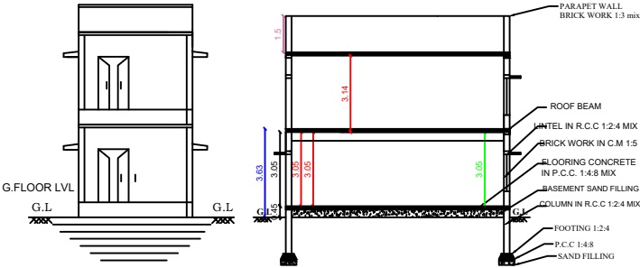
ELEVATION (South Facing)
