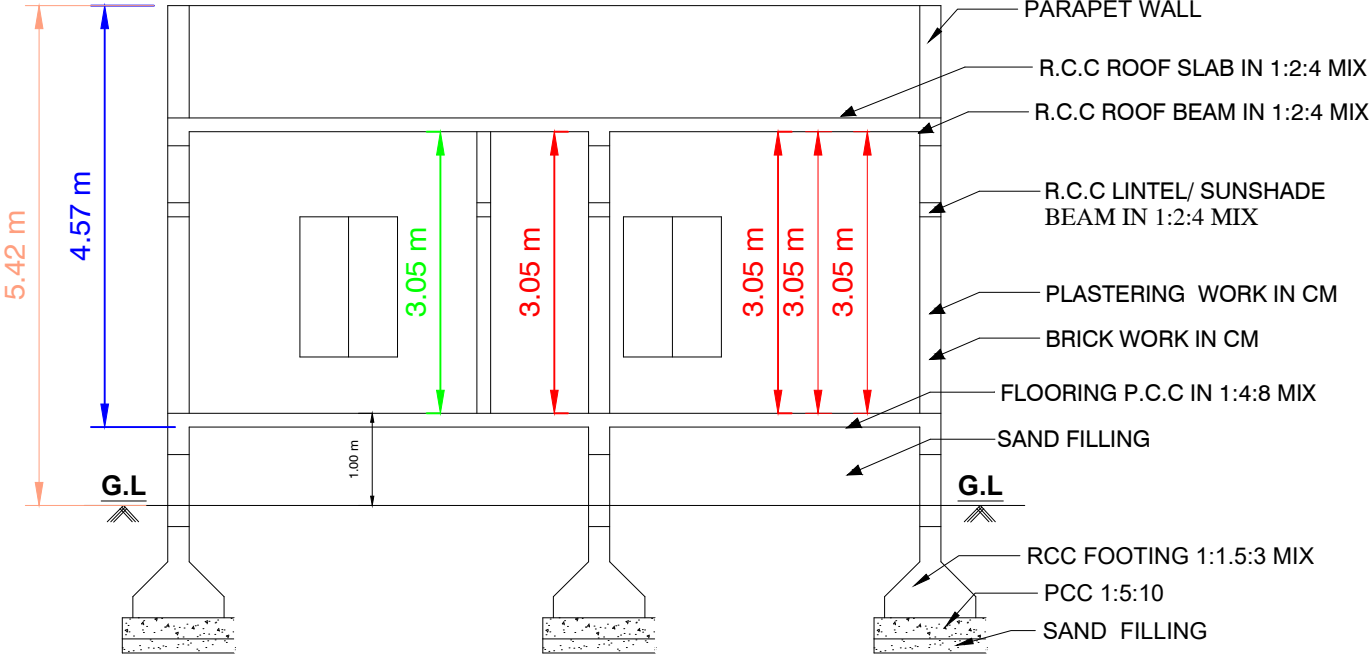
SECTION"AB"
