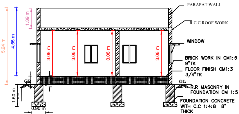
SECTION " AB "
