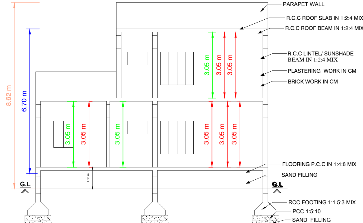
SECTION"AB"
