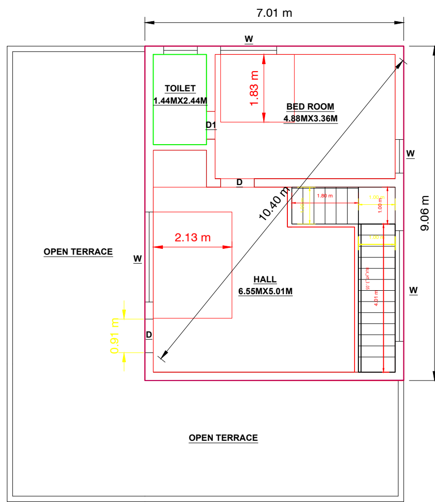
FIRST FLOOR
