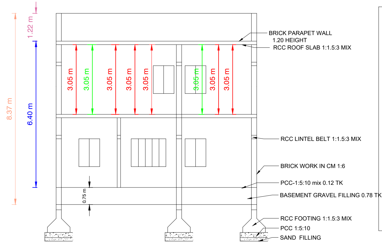
SECTION"AB"
