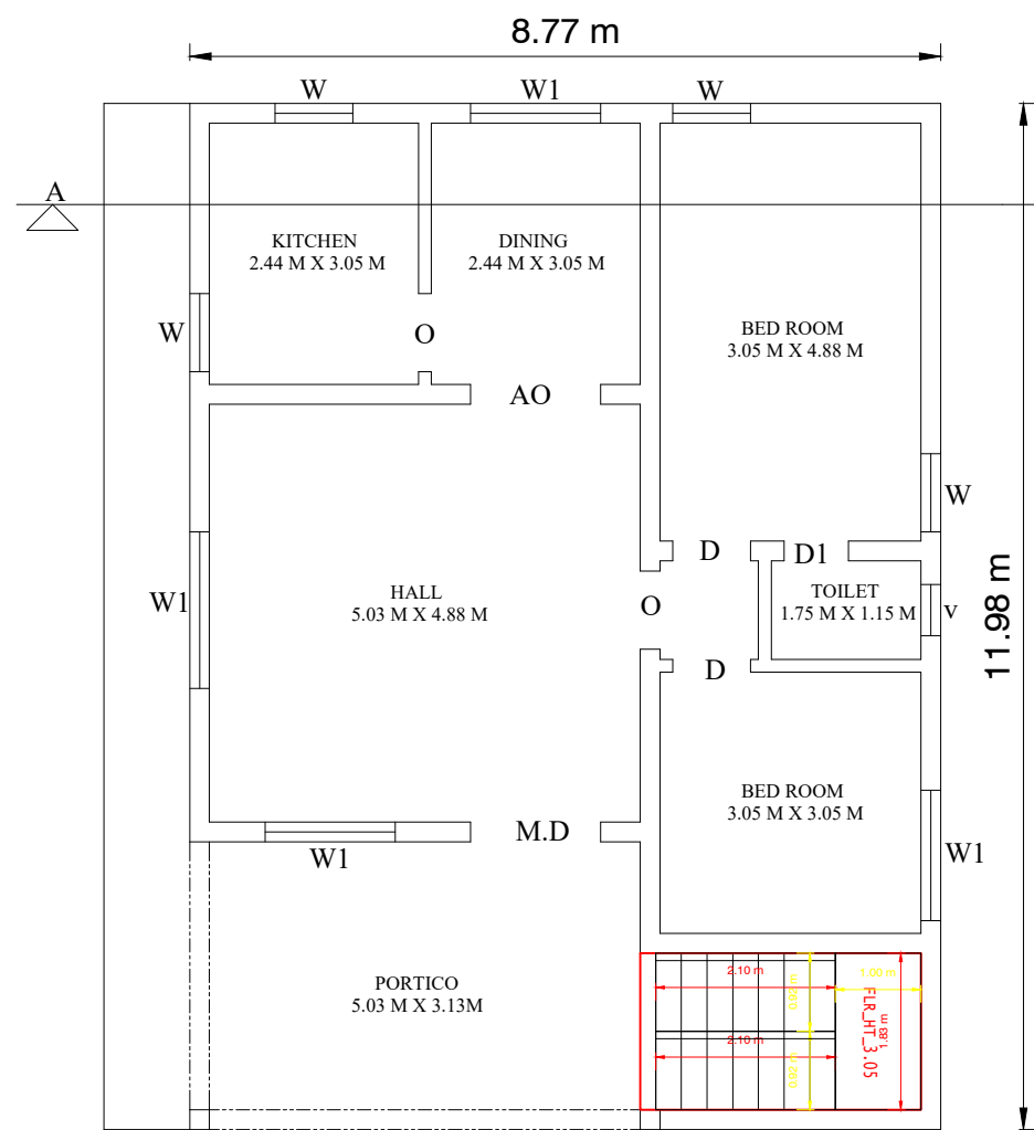
EXI- G.F PLAN [NORTH FACING]
