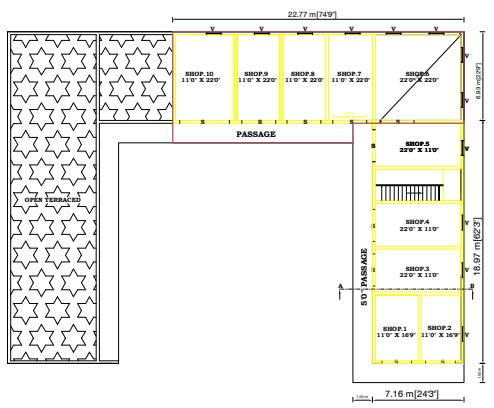
PROPOSED FIRST FLOOR [SOUTH PART] -COMMERCIAL - PLAN
