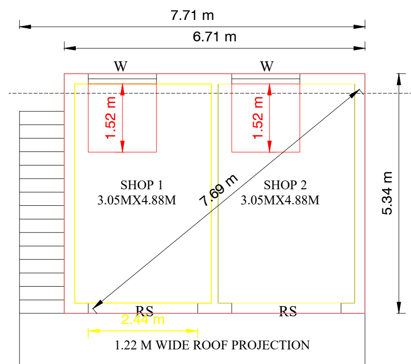
COMMERCIAL - PLAN
