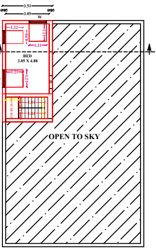
PROPOSED SECOND FLOOR
