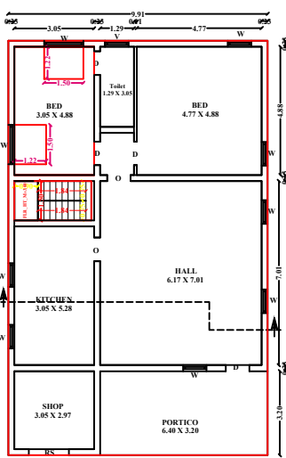
EXISTING GROUND FLOOR
