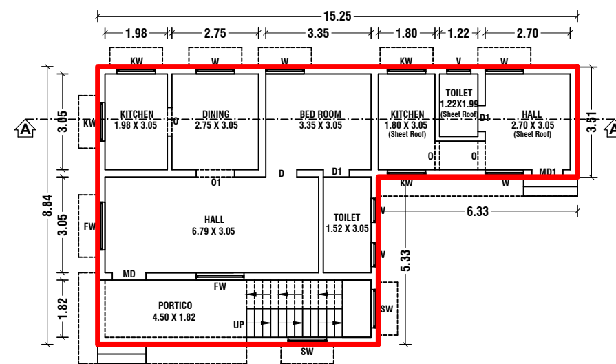
NORTH FACING GROUND FLOOR PLAN
