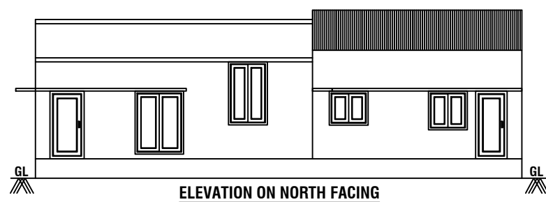
ELEVATION ON NORTH FACING
