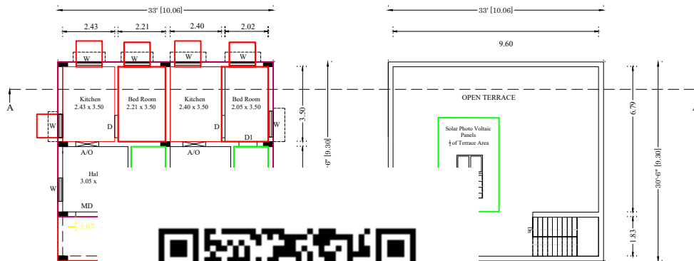
F FLOOR PLAN
