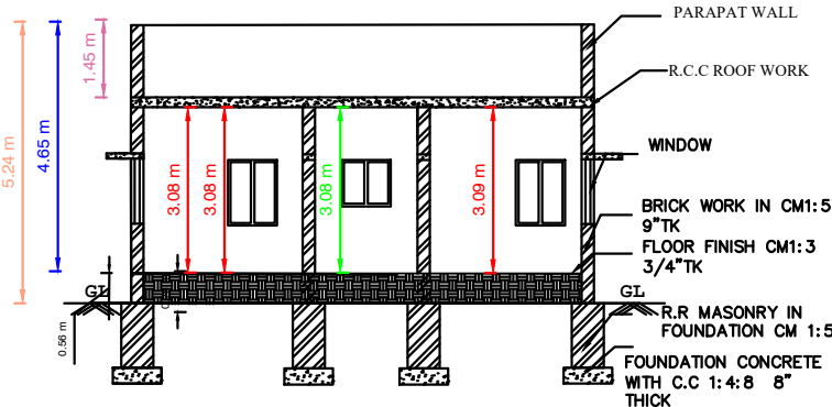
SECTION " AB "
