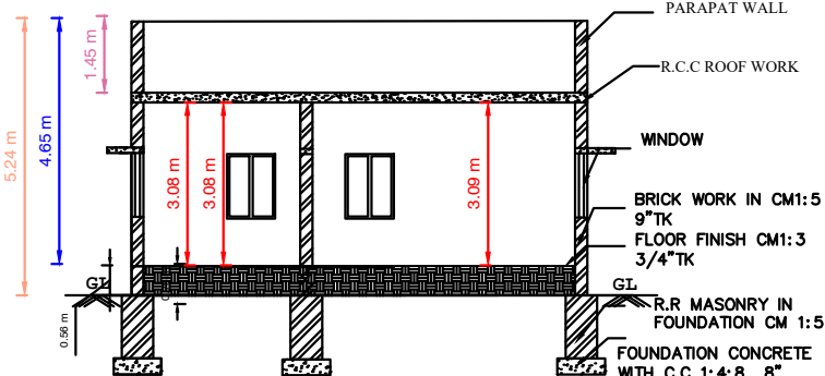
SECTION " AB "
