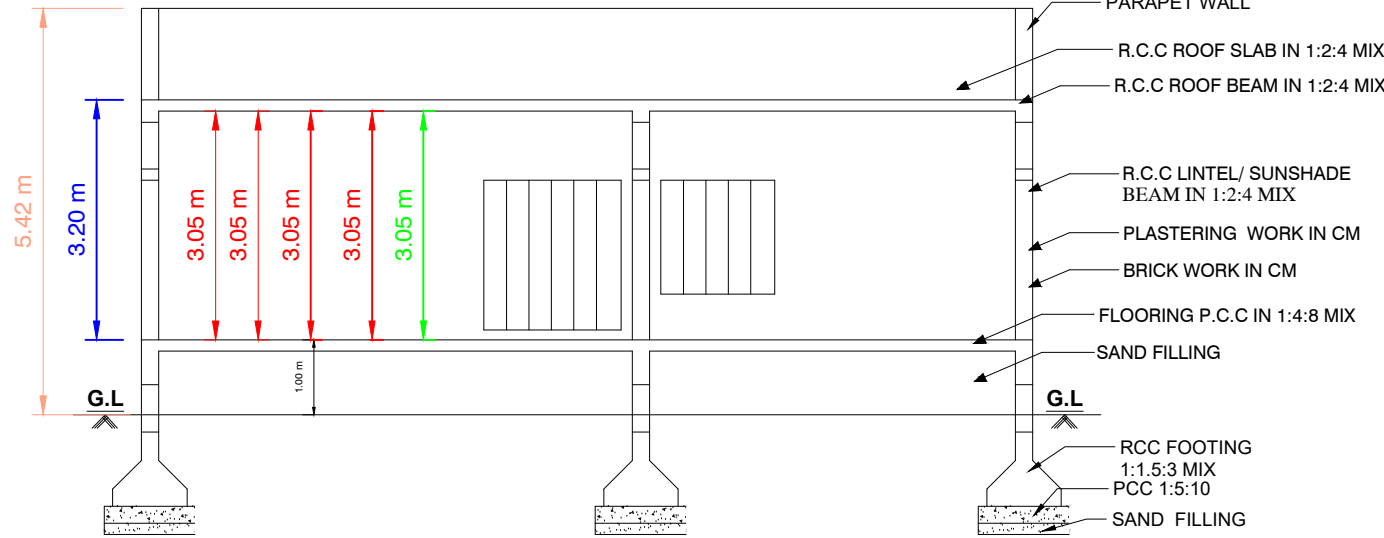
SECTION"AB"
