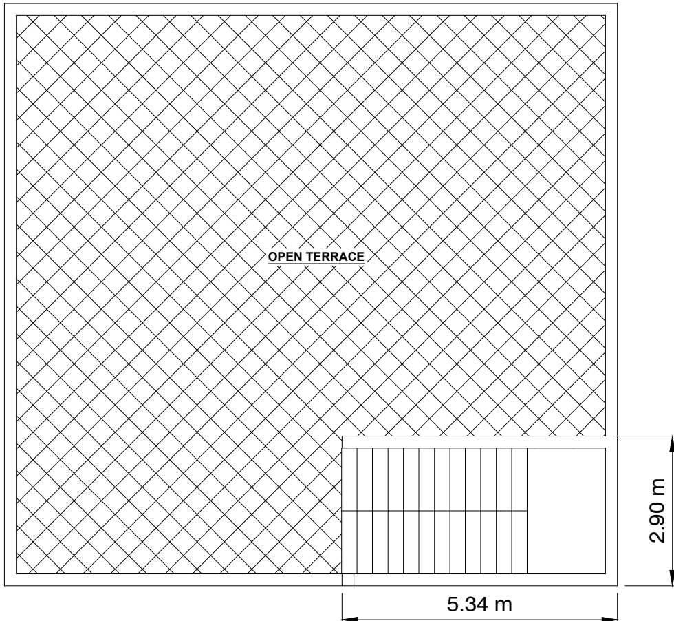
TERRACE PLAN
