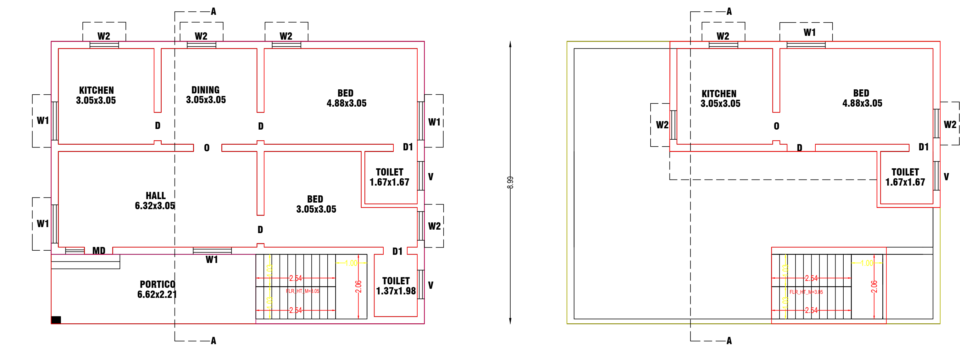
GROUND FLOOR PLAN (SCALE 1:100)
