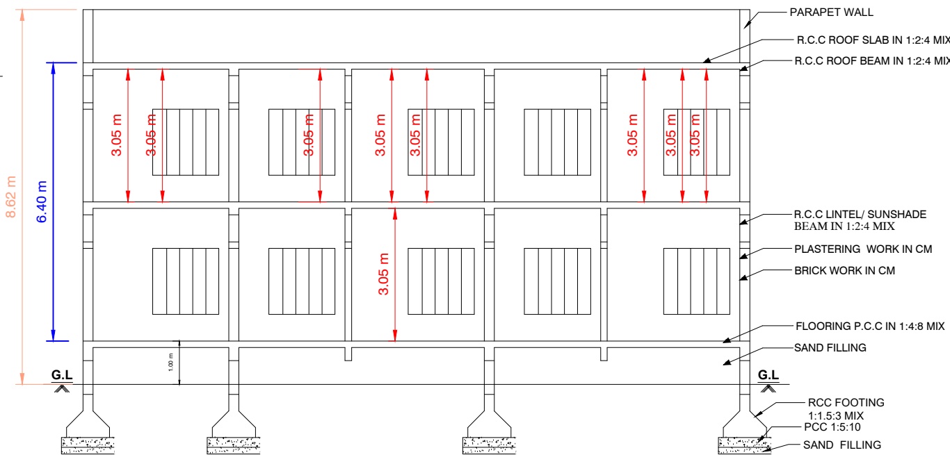
SECTION "AB"
