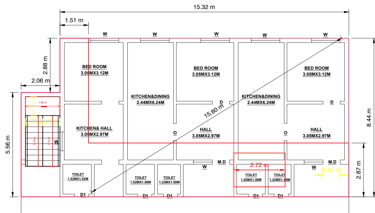
EXI & PRO GROUND FLOOR
