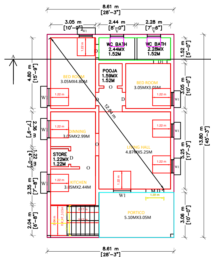
GROUND FLOOR PLAN ENTRANCE FACING TO EAST
