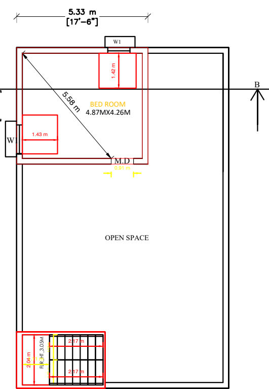
FIRST FLOOR PLAN ENTRANCE FACING TO EAST
