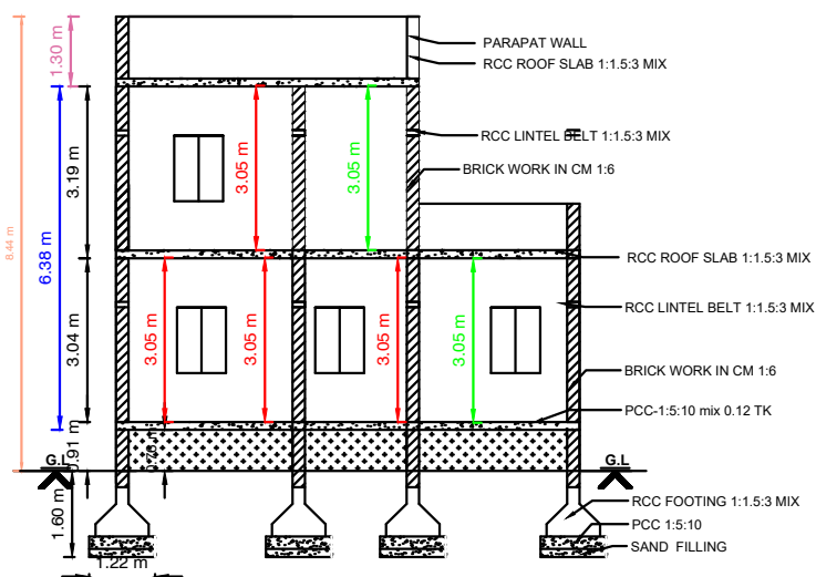
SECTION "AB"
