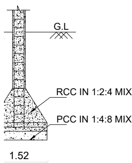
OF RCC COLUMN SCALE 1:50
