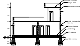
SECTION ON "ABC"
