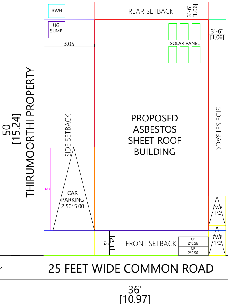
SITE PLAN (1:100)
