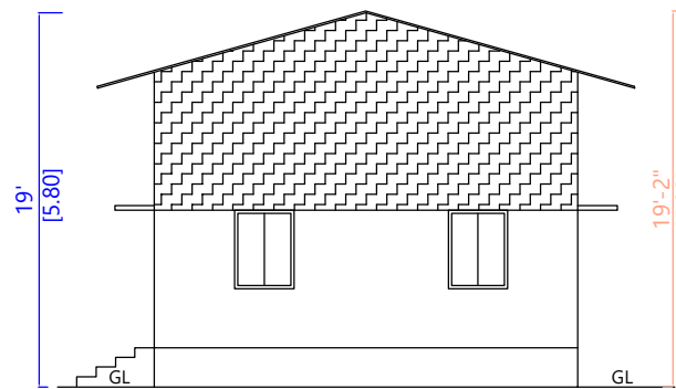
FRONT ELEVATION (WEST SIDE VIEW)
