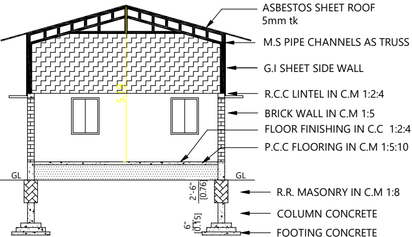
CROSS SECTION "AB"
