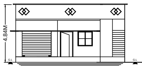
FRONT ELEVATION
